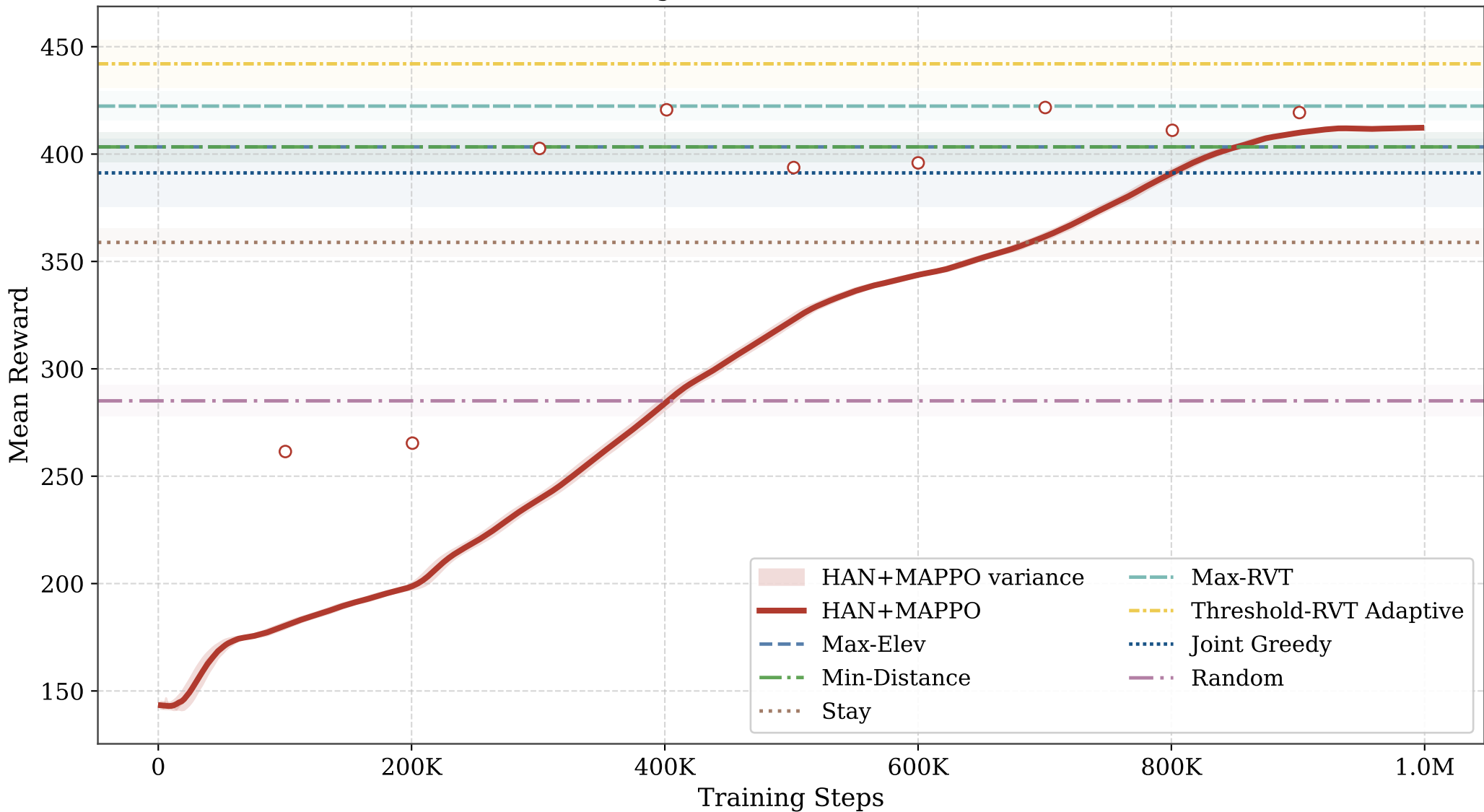
Reward Convergence vs. Heuristic Baseline Levels
