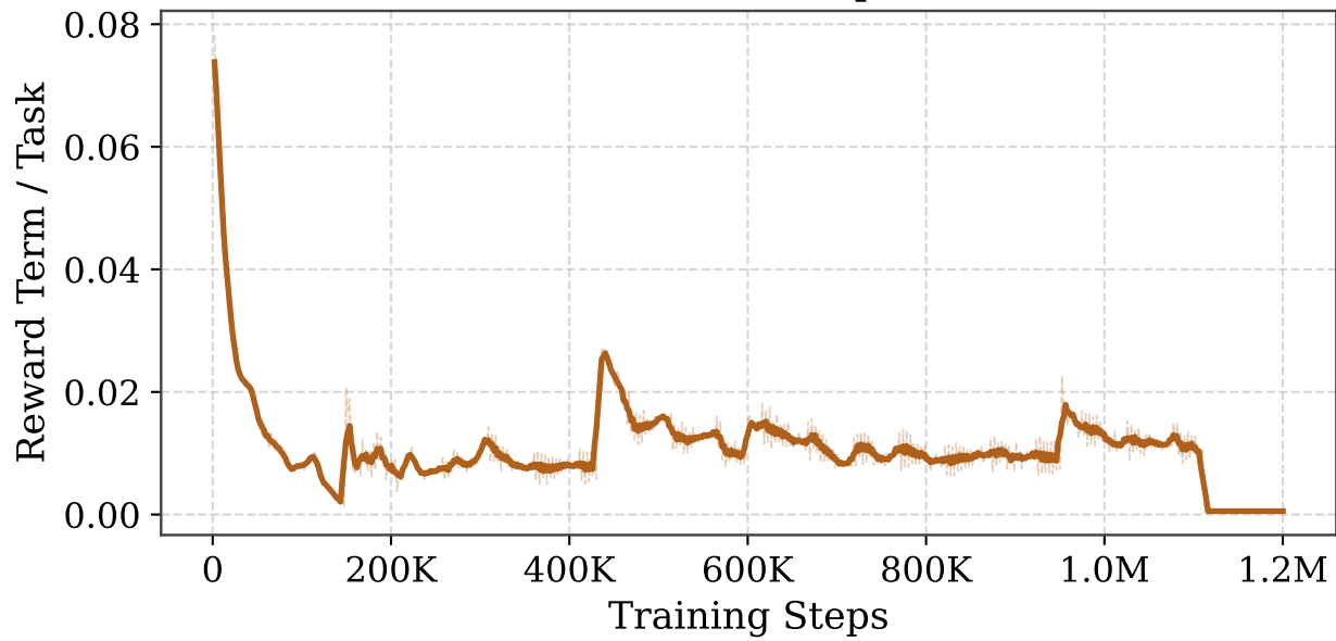
Enqueue Reward per Task
