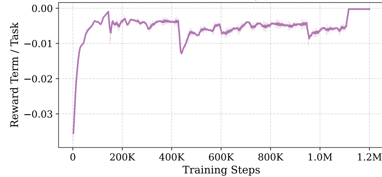
Queue-Full Penalty per Task
