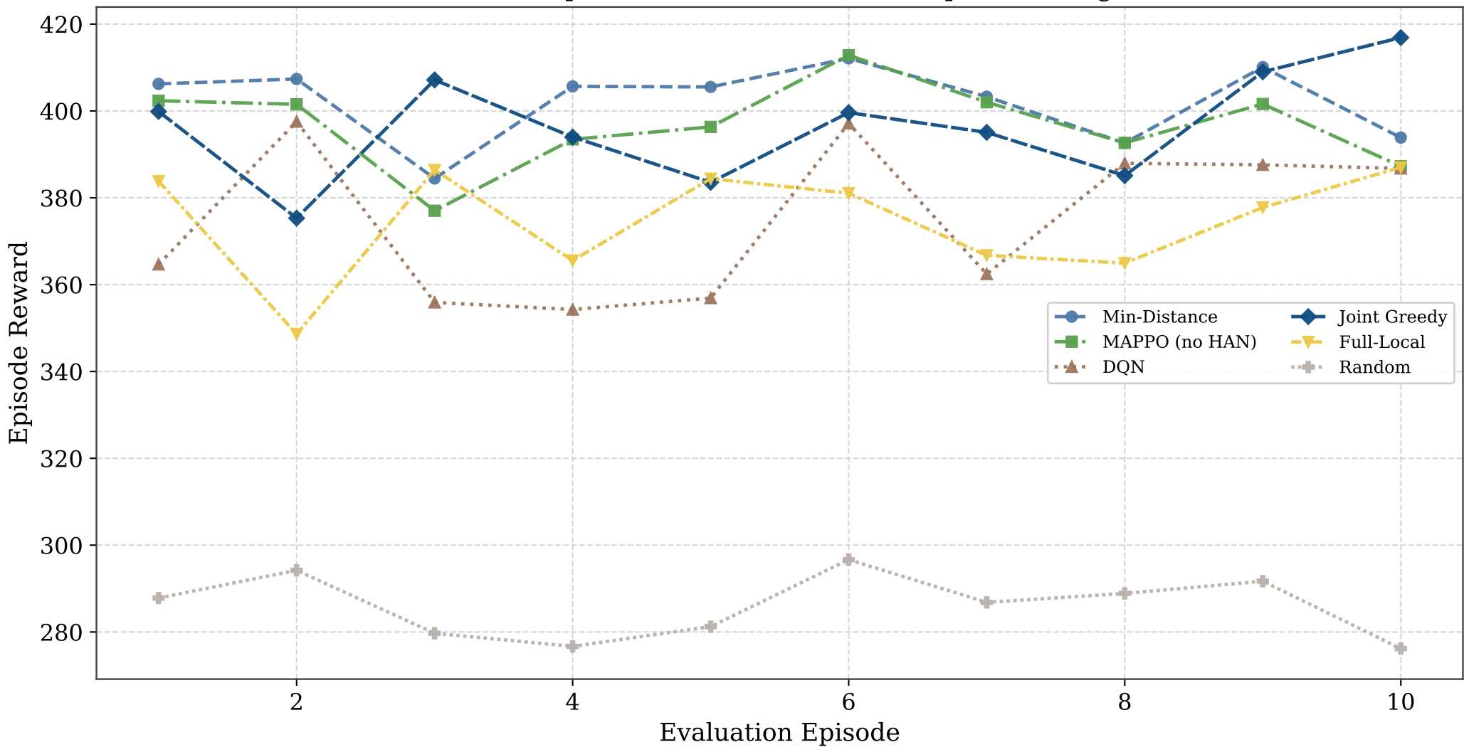
Baseline Reward Comparison Across Evaluation Episodes (Higher is better)
