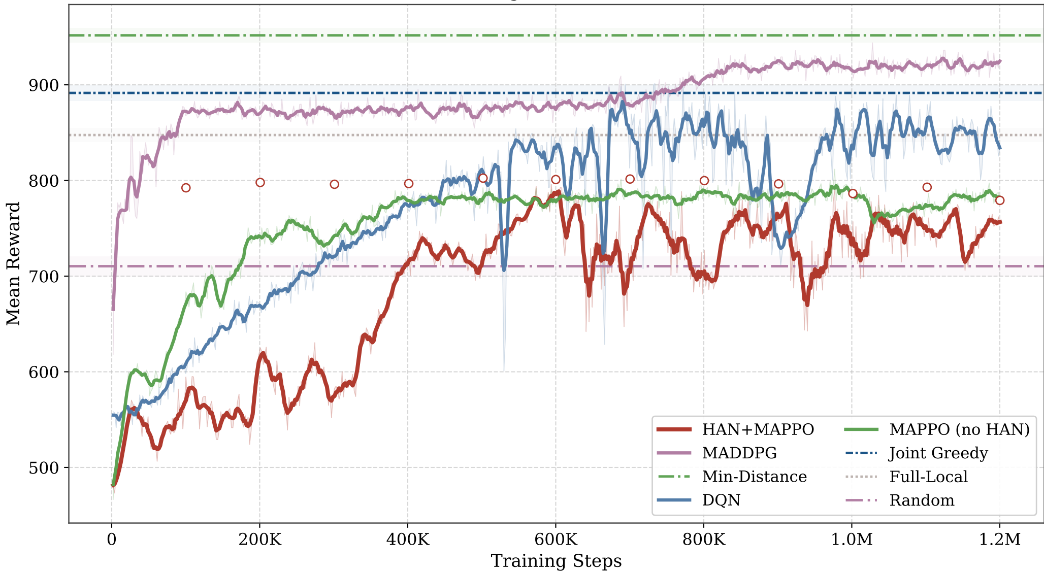
Reward Convergence vs. Baseline Levels
