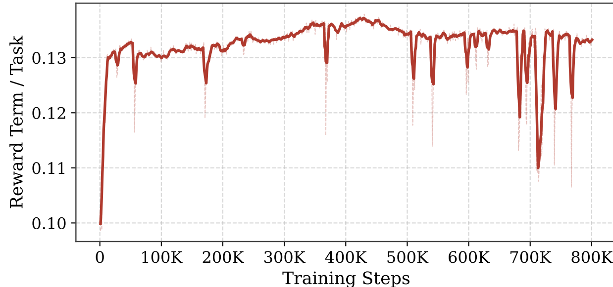
Service Interruption Penalty per Task
