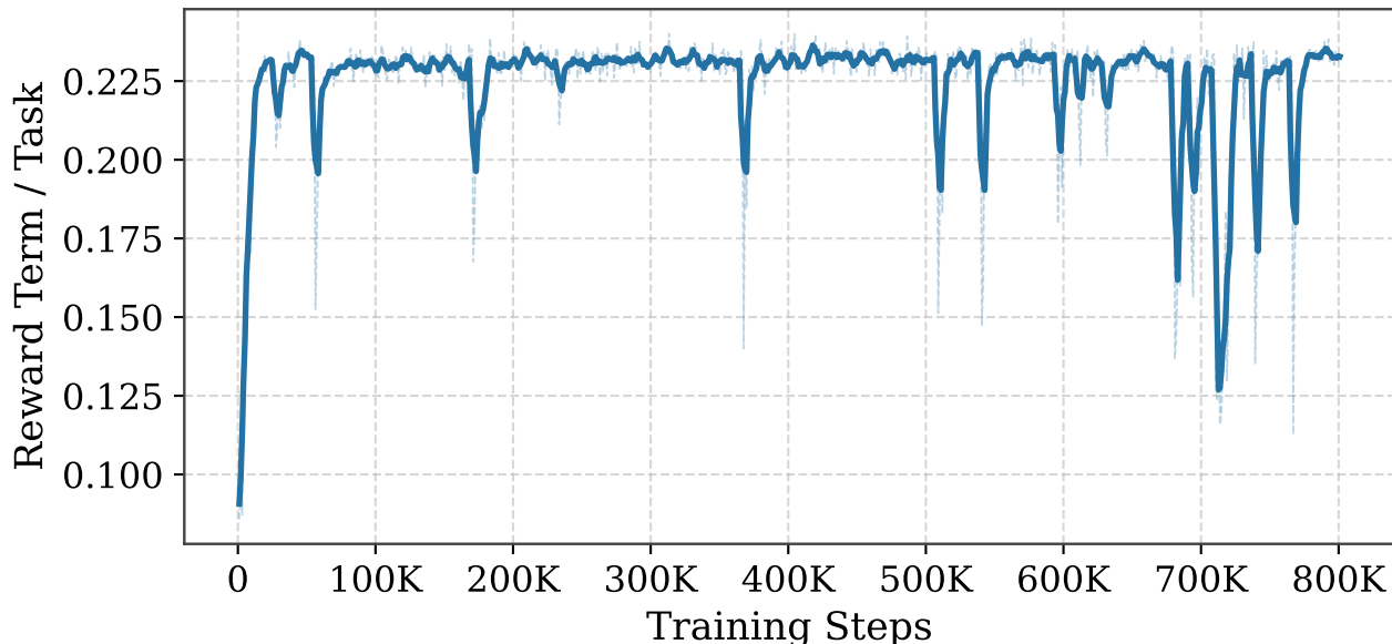
Handover Reward per Task
