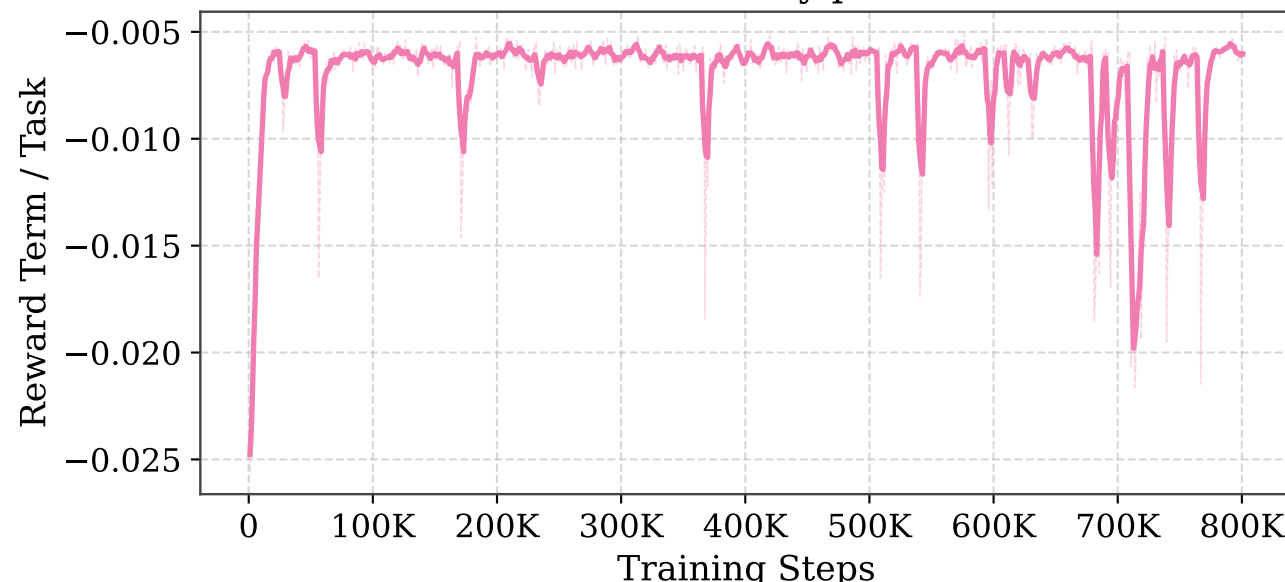
Handover Cost Penalty per Task
