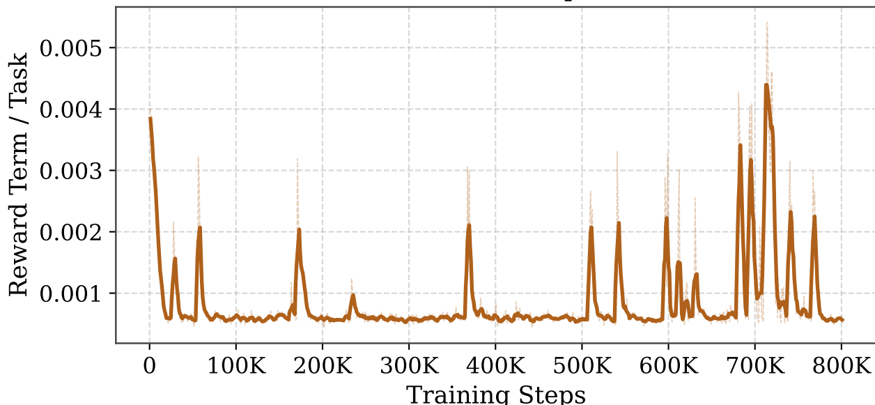
Enqueue Reward per Task
