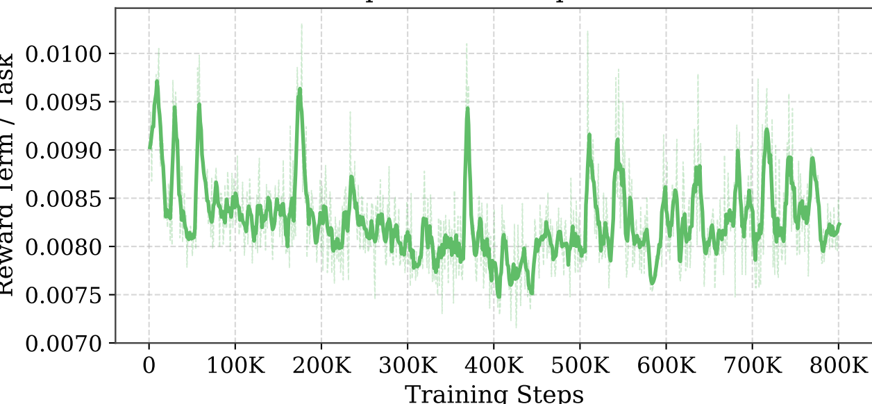
Failed Handover Penalty per Task
