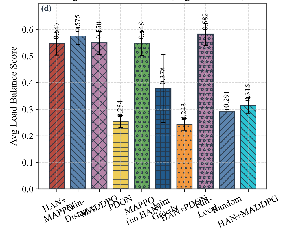
Avg Load Balance Score (Higher is better)
