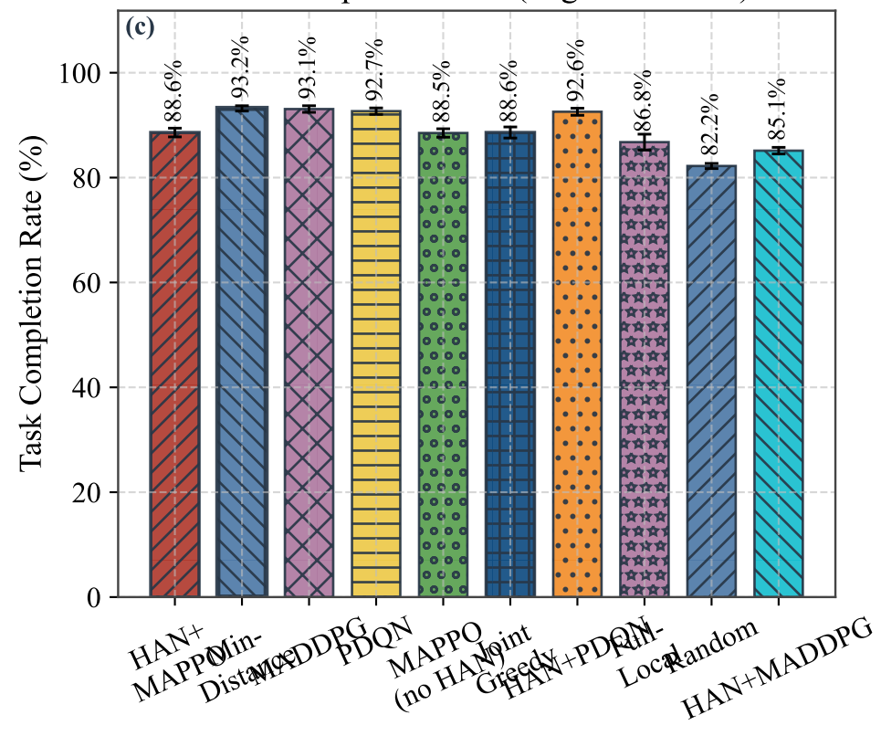
Task Completion Rate (Higher is better)
