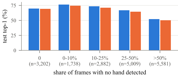
(b) accuracy vs. missing hands
