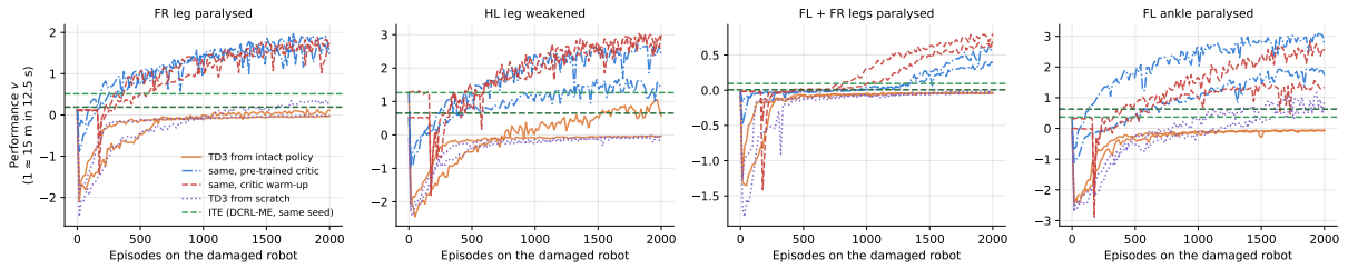
Figure 7: TD3 on the damaged robot (two seeds each): from scratch, from the best intact DCRL-ME policy, and from the same policy with a critic warm-up or a pre-trained critic, against the performance of the gait found by ITE on the DCRL-ME repertoire of the same seed (dashed lines).
