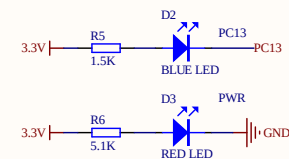
指示灯 Indicator light
