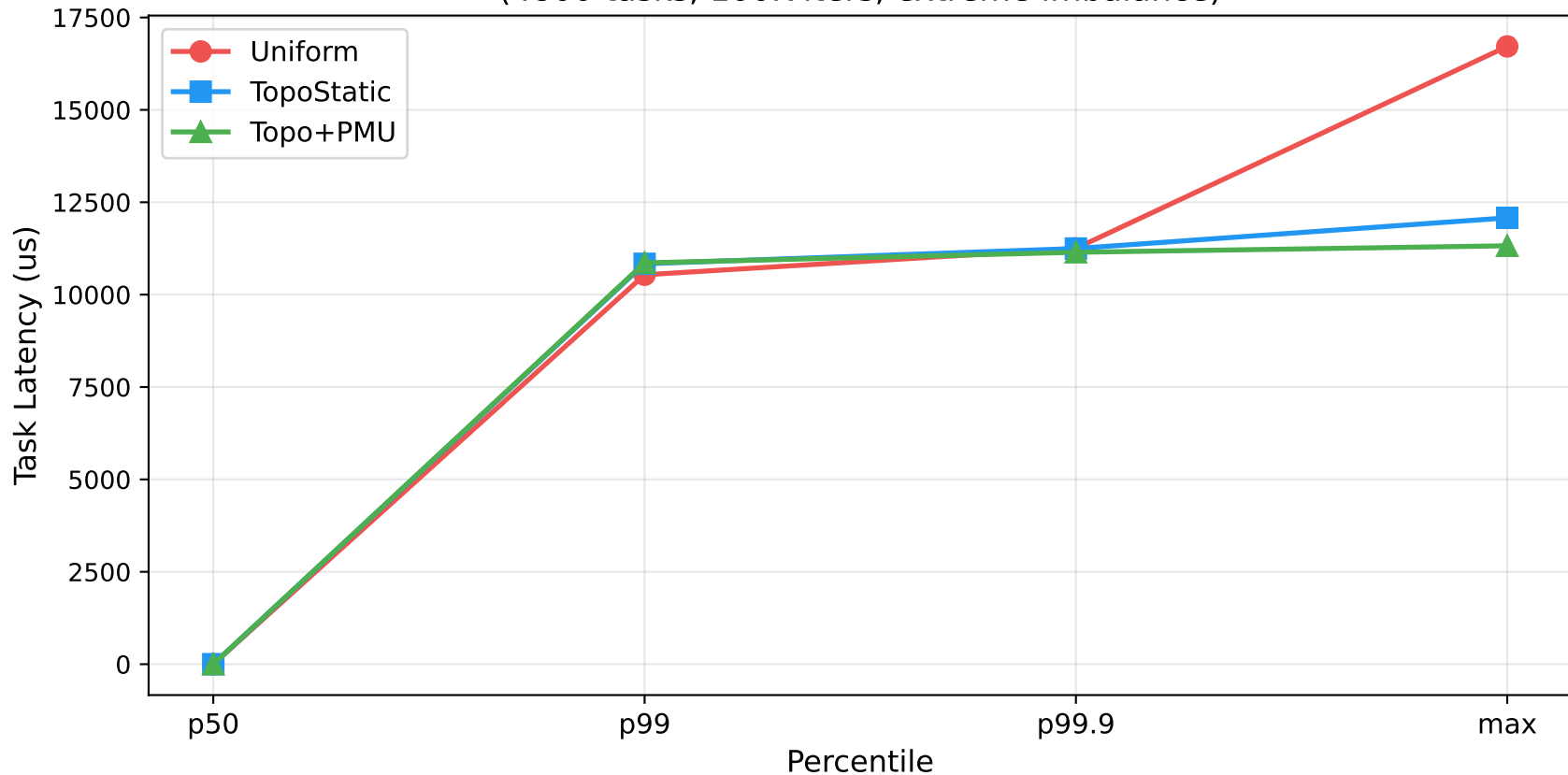
Latency Percentile Ladder — HFT Burst Config (4800 tasks, 100K iters, extreme imbalance)
