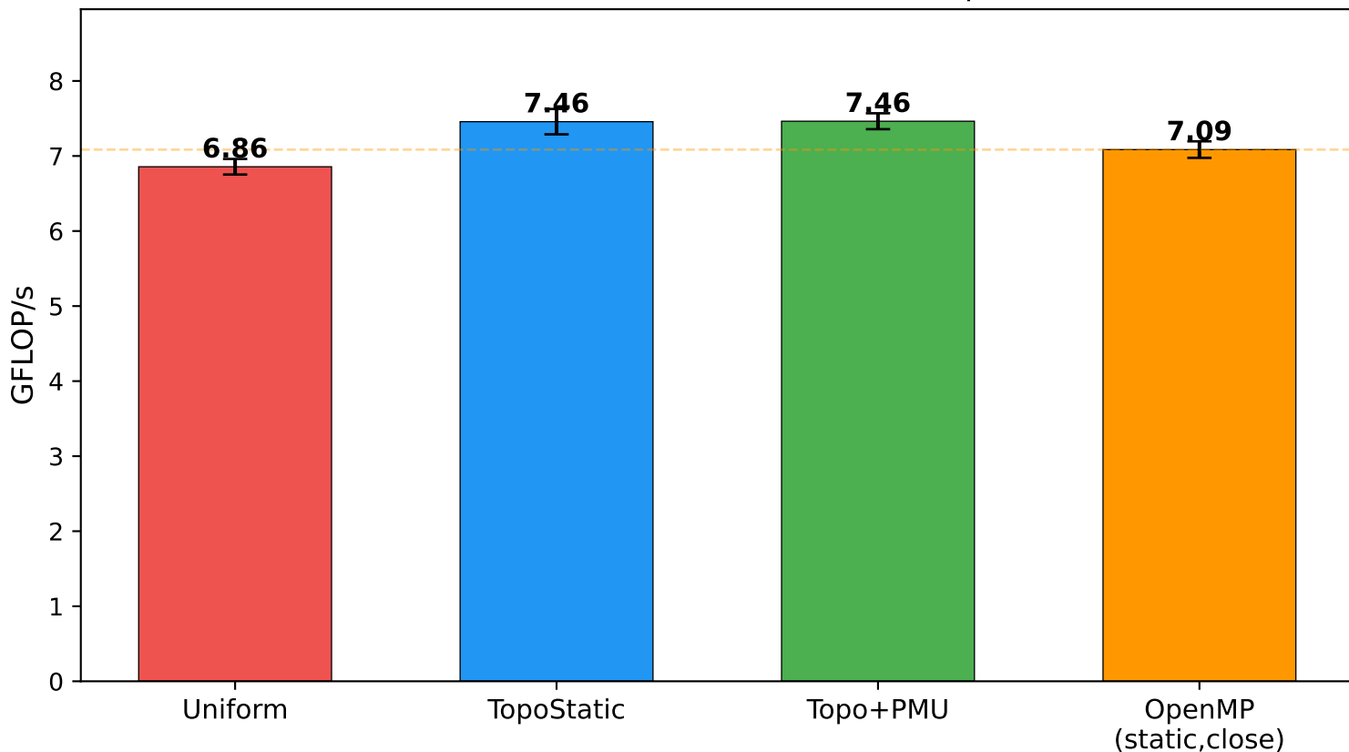
SpMV Performance: audikw_1 (943K rows, 77M nnz) 2x Xeon E5-2690v3, 24 cores, 20 outer reps, 5 trials
