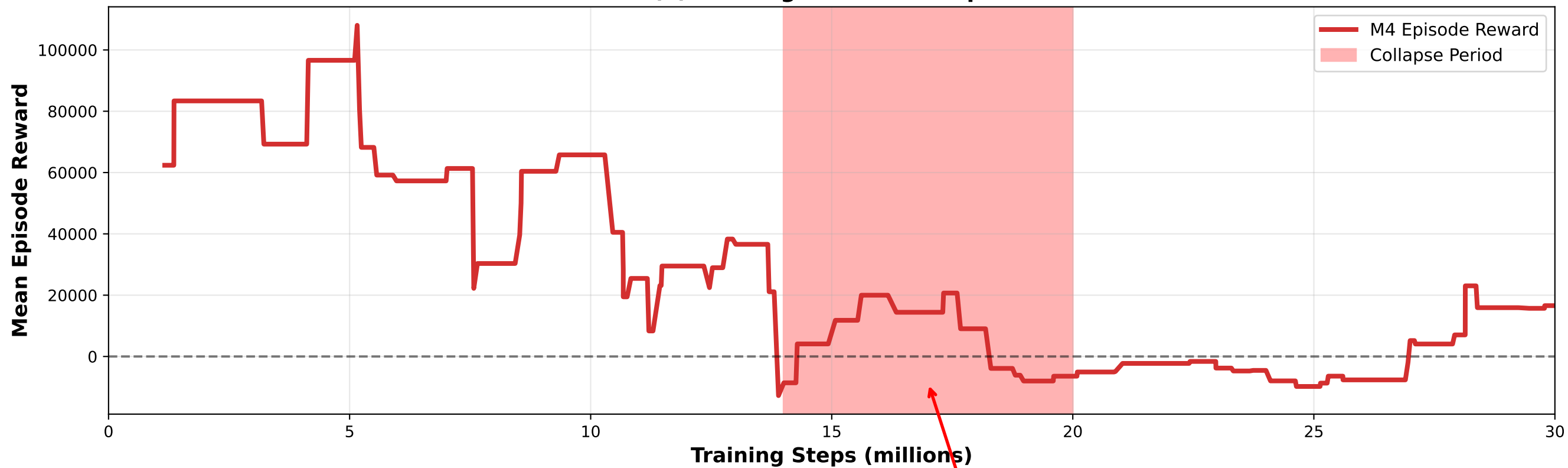
(a) Training Reward Collapse
