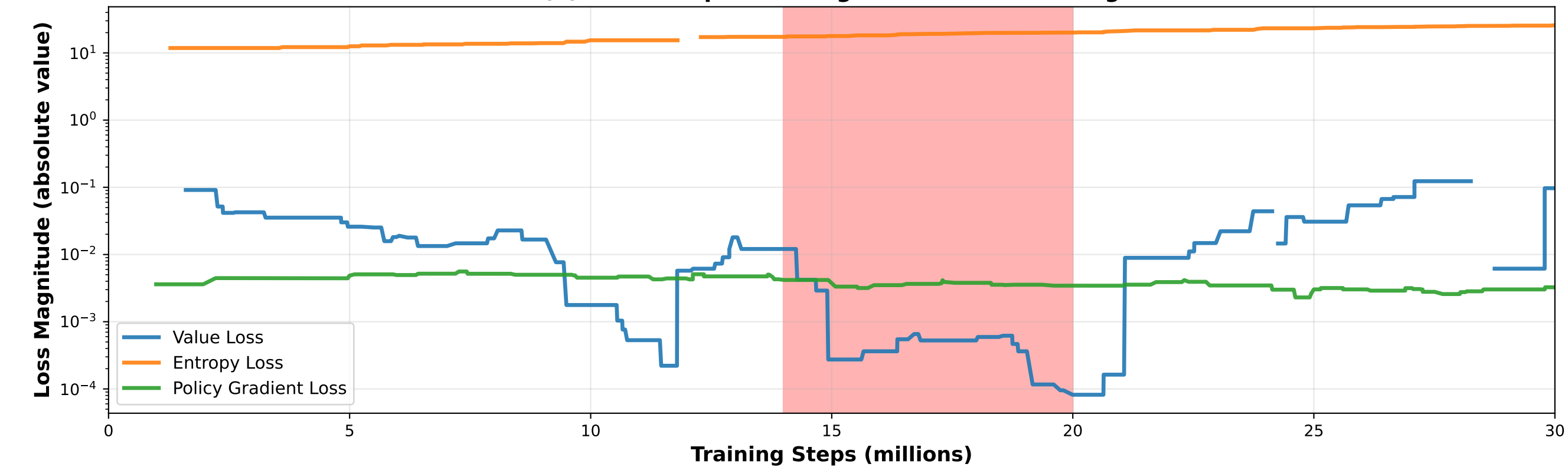
(b) Loss Component Magnitudes Over Training
