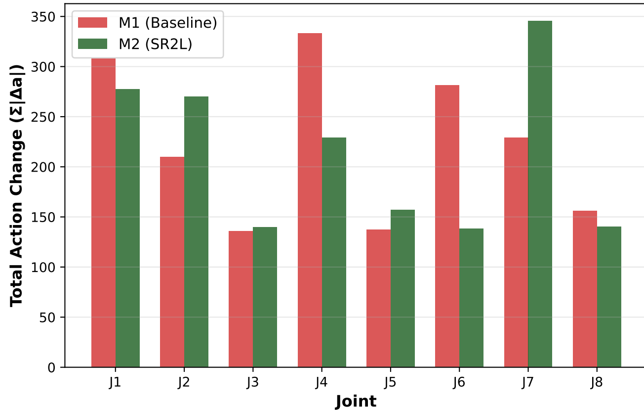
Per-Joint Action Changes (Lower = Smoother)
