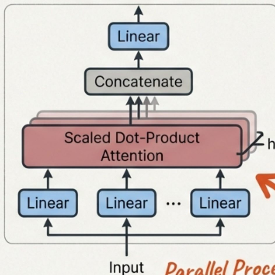
Multi-Head Attention
