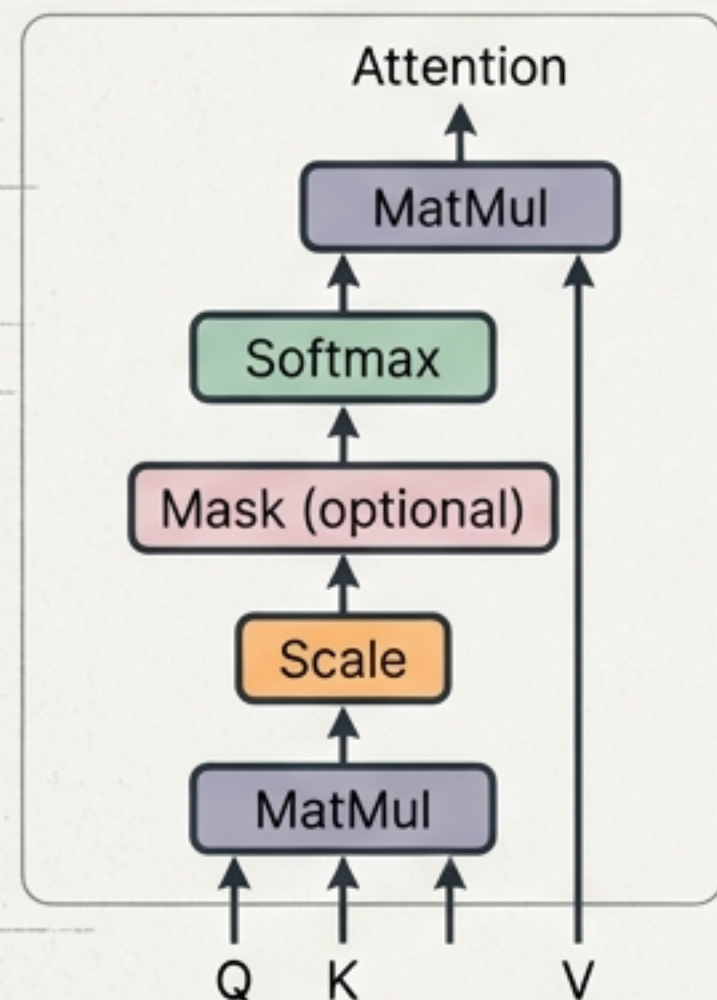
Scaled Dot-Product Attention
