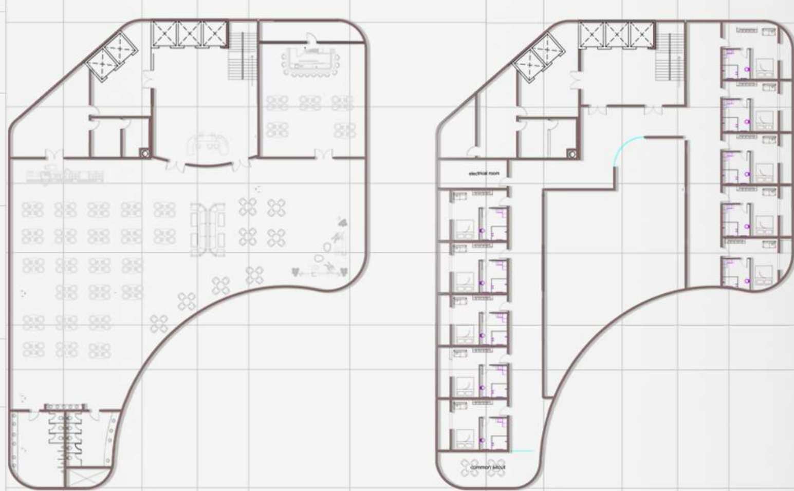
Hotel floor plan
