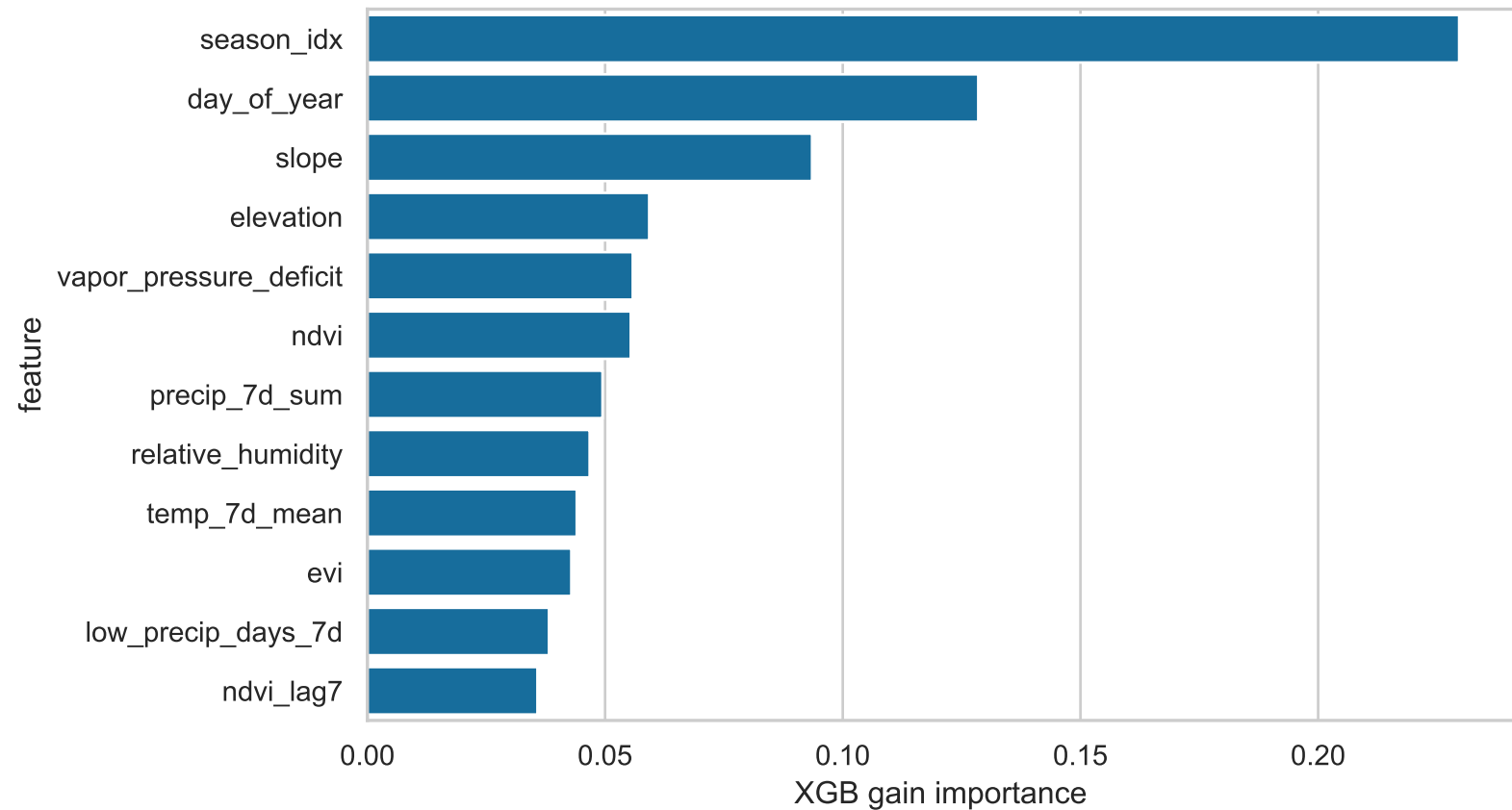
Top feature importances
