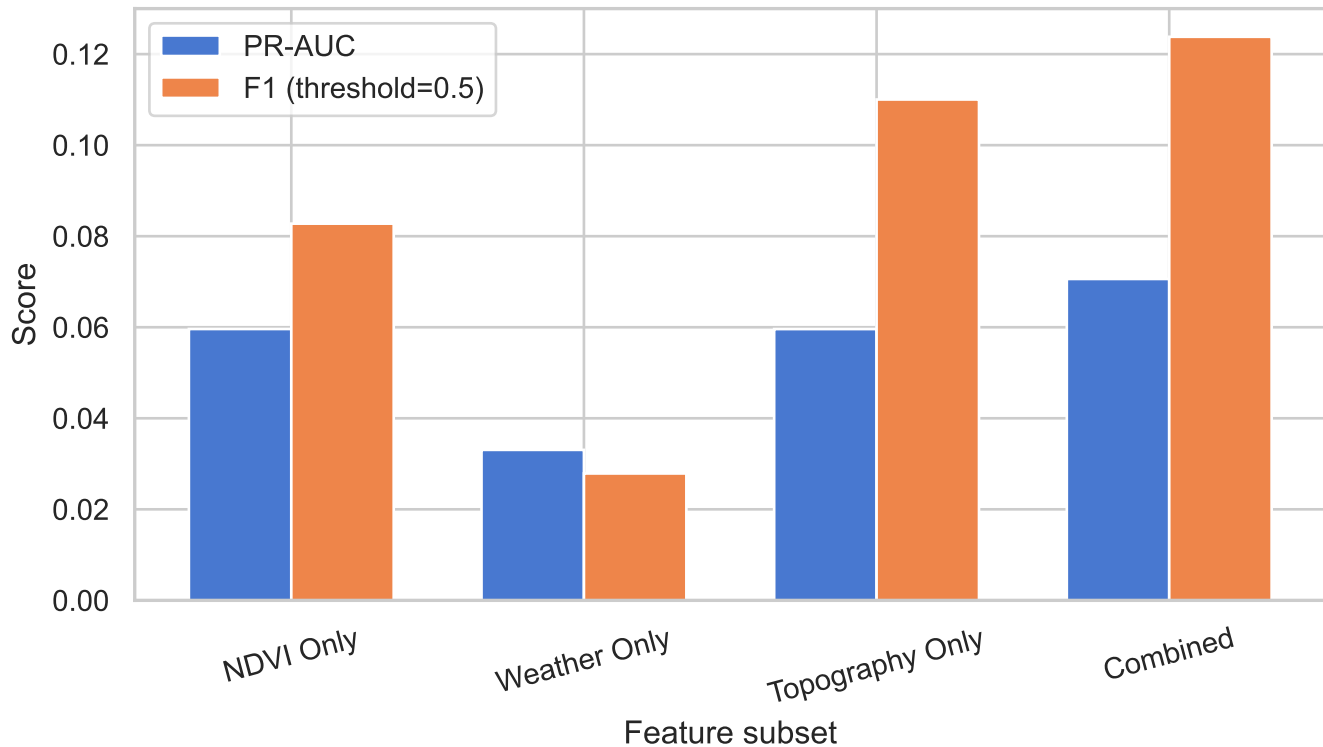
RQ2 — Feature-set ablation (XGB holdout)
