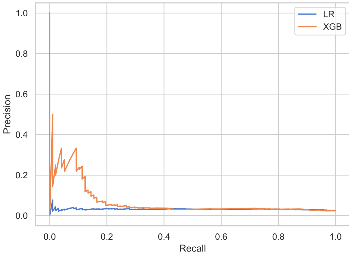
RQ4 — PR curves (balanced models, holdout)
