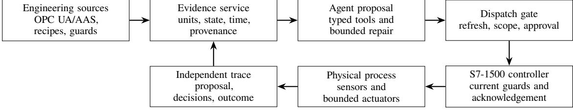
Fig. 1. Proposed supervisory architecture. Evidence supports the agent; dispatch and PLC checks retain current-condition authority. This is a design, not evidence of a completed physical trial.
