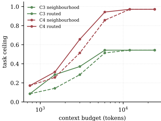
(b) intent routing vs. budget
