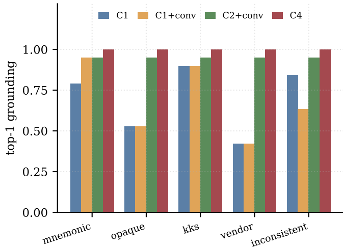
(a) accuracy vs. naming convention
