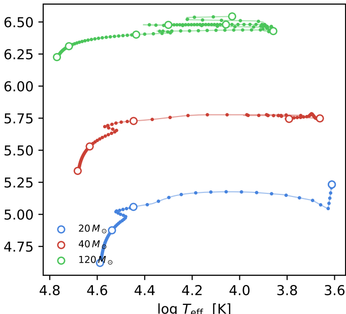
SMC: MIST EEP placement
