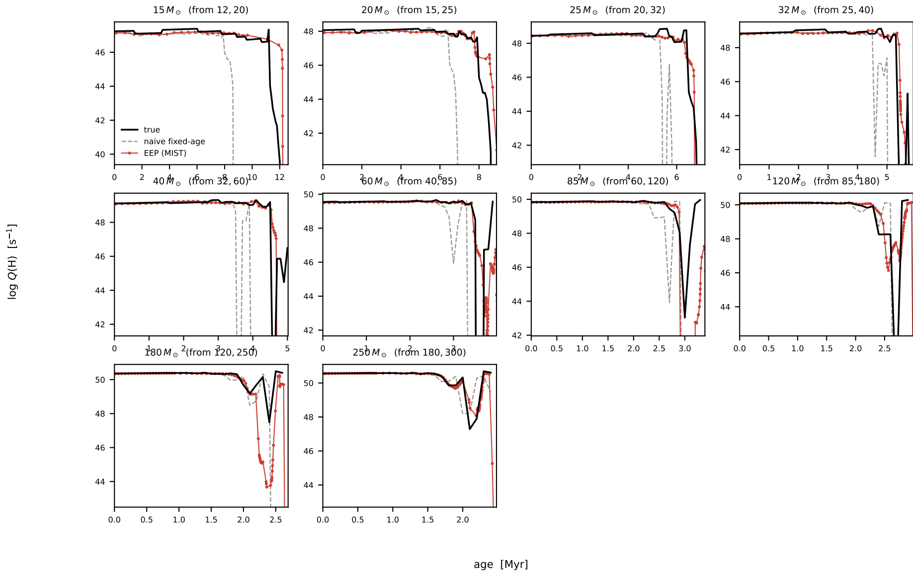
LMC: leave-one-out log Q(H) [ s^{-1} ] reconstruction, all 10 interior masses
