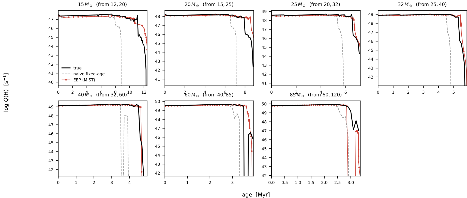
SMC: leave-one-out log Q(H) [ s^{-1} ] reconstruction, all 7 interior masses
