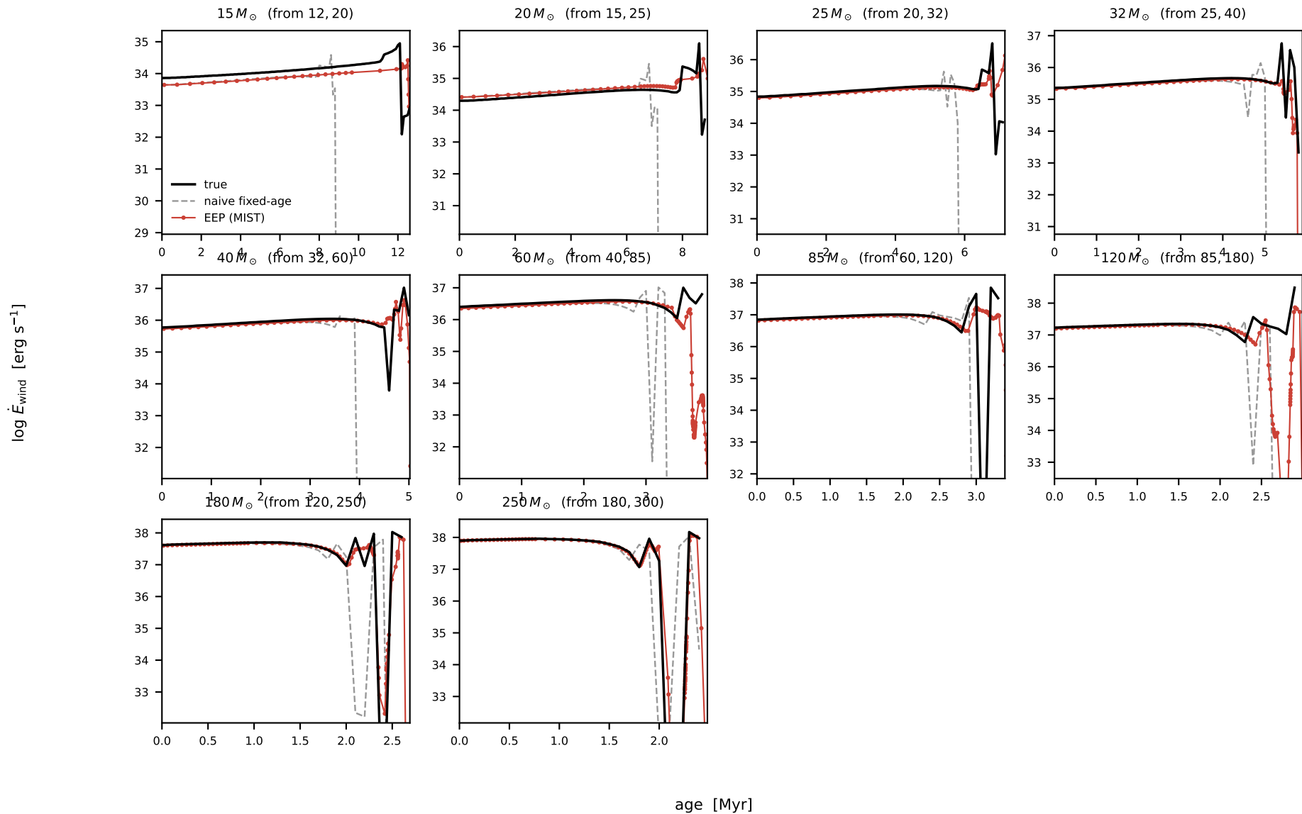
LMC: leave-one-out \log \dot{E}_{\text{wind}} [erg s -1 ] reconstruction, all 10 interior masses
