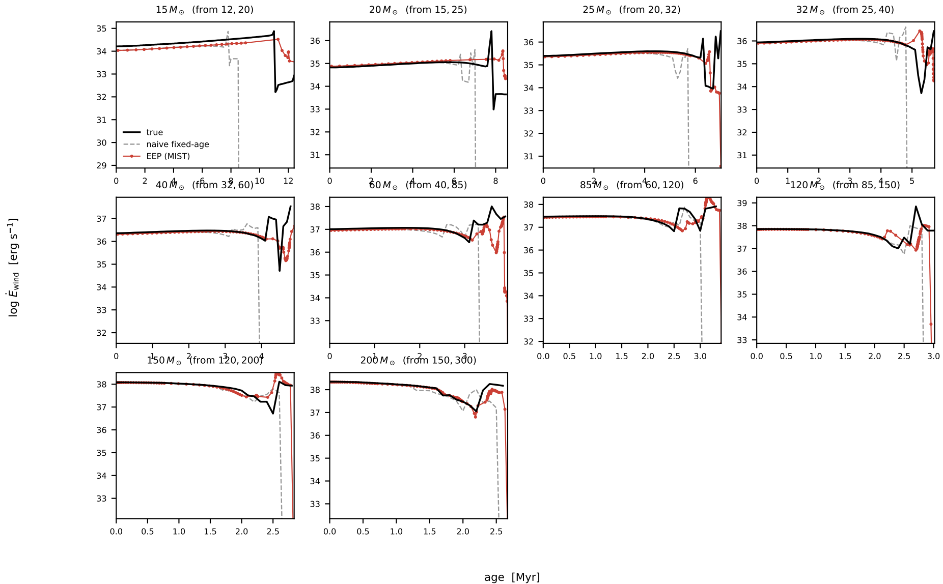
MWC: leave-one-out \log \dot{E}_{\text{wind}} [erg s -1 ] reconstruction, all 10 interior masses
