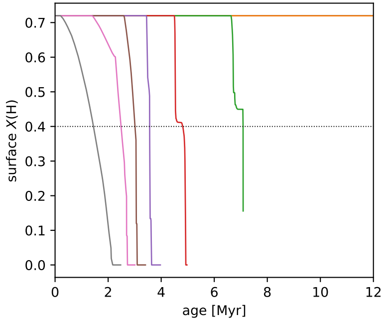
surface H (WR onset at 0.4)
