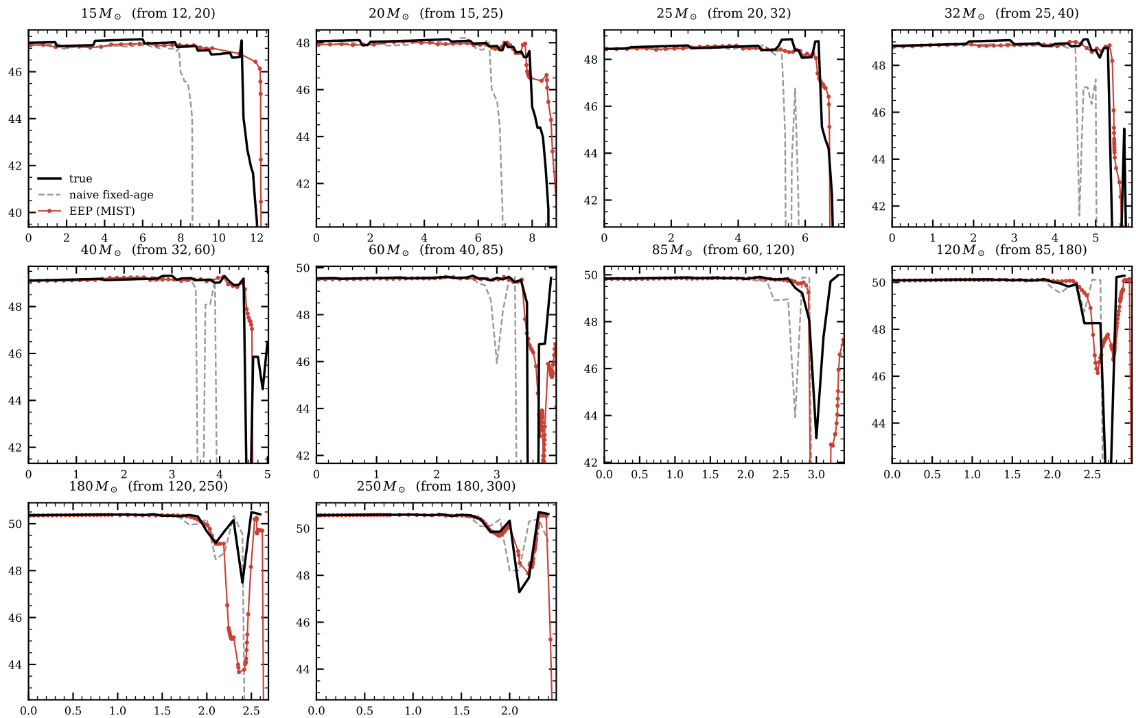
LMC: leave-one-out log Q(\text{H}) [ \text{s}^{-1} ] reconstruction, all 10 interior masses
