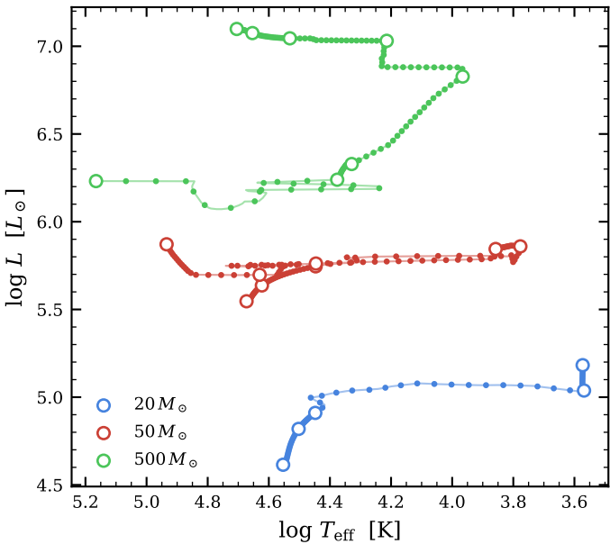
MW: MIST EEP placement
