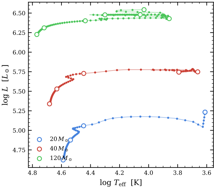
SMC: MIST EEP placement
