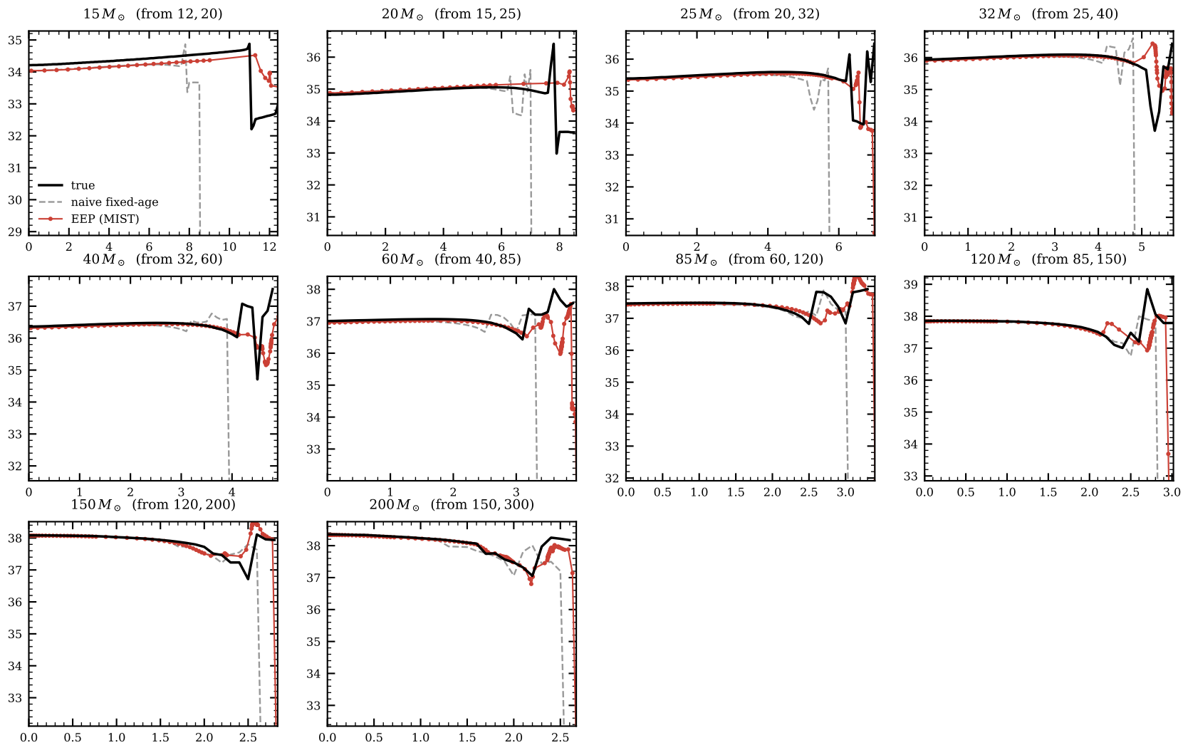
MWC: leave-one-out \log \dot{E}_{\text{wind}} [\text{erg s}^{-1}] reconstruction, all 10 interior masses
