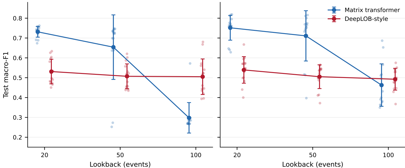
Horizon 10 events
