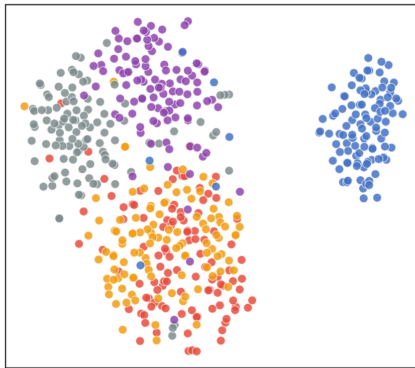
JEPA-SIGReg (25Hz)
