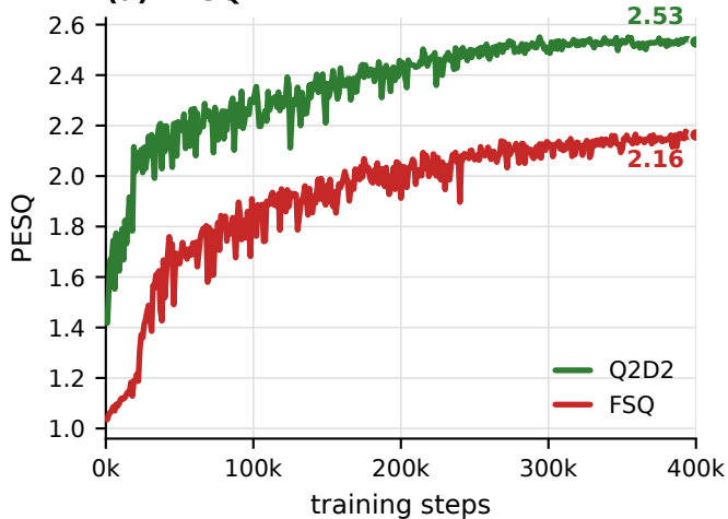
(a) PESQ
