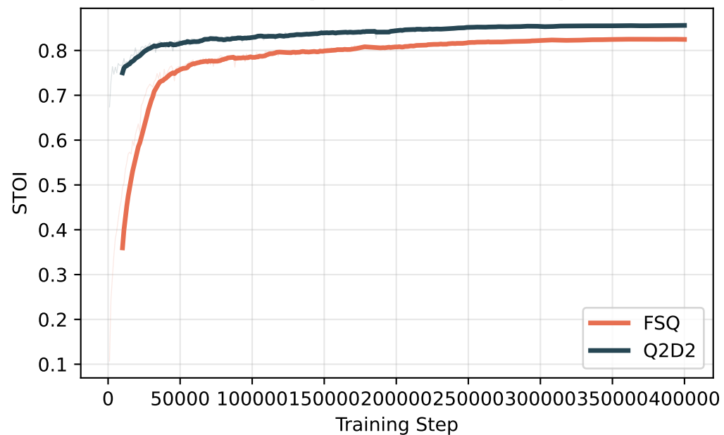
STOI: Q2D2 +0.031 over FSQ
