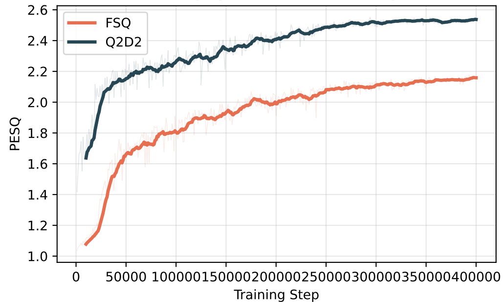
PESQ: Q2D2 +0.368 over FSQ
