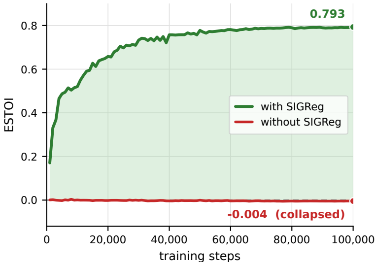
(a) Q2D2 codec training (25 Hz, cd32)
