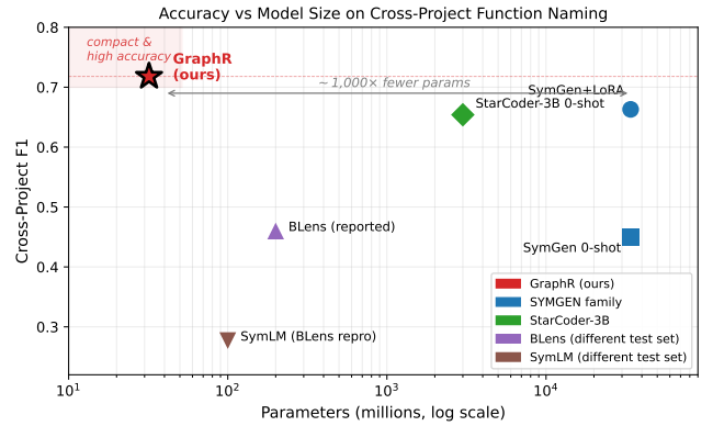
Figure 5: Accuracy versus parameter count on cross-project function naming (log scale). GRAPHR occupies the top-left corner: high cross-project F1 with two-to-three orders of magnitude fewer parameters than the LLM-based baselines. Markers in the same color reproduce on our 4-package cross-project test set; lighter-colored markers (BLens, SymLM) report numbers from the BLens’25 reproduction on Punstrip and are shown for literature-anchor context.
