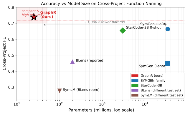
Figure 5: Accuracy versus parameter count on cross-project function naming (log scale). GRAPHR (25M, 0.738 adaptive-gate F1 on cross-project) occupies the top-left corner: high cross-project F1 with two-to-three orders of magnitude fewer parameters than the LLM-based baselines. Markers in the same color reproduce on our cross-project test set; lighter-colored markers (BLens, SymLM) report numbers from the BLens’25 reproduction on Punstrip and are shown for literature-anchor context.
