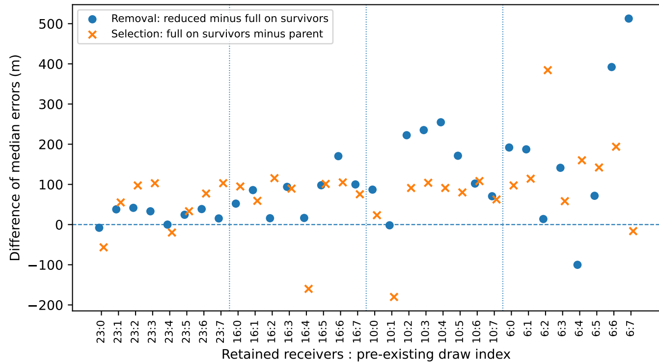
Fingerprint (k=3) — existing draw-by-draw decomposition
