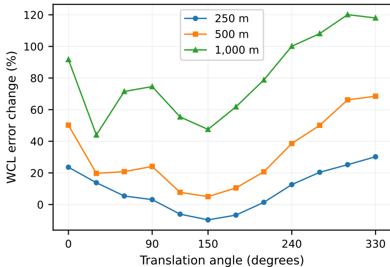
(a) Directional response on R29
