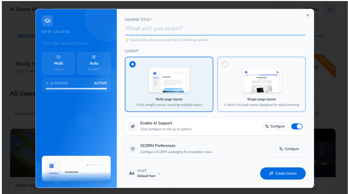
Figure — Create Course dialog — title, layout, AI Support, SCORM, Font
