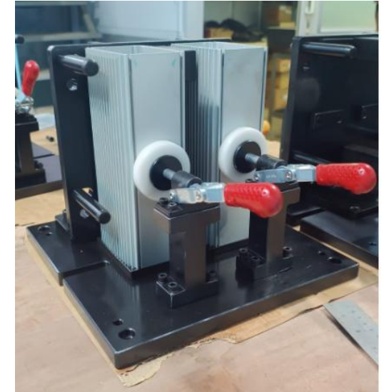
Toggle clamping VMC fixture:
