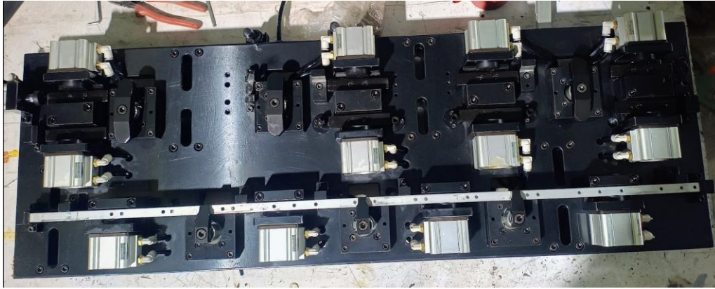
Pneumatic VMC fixture:
