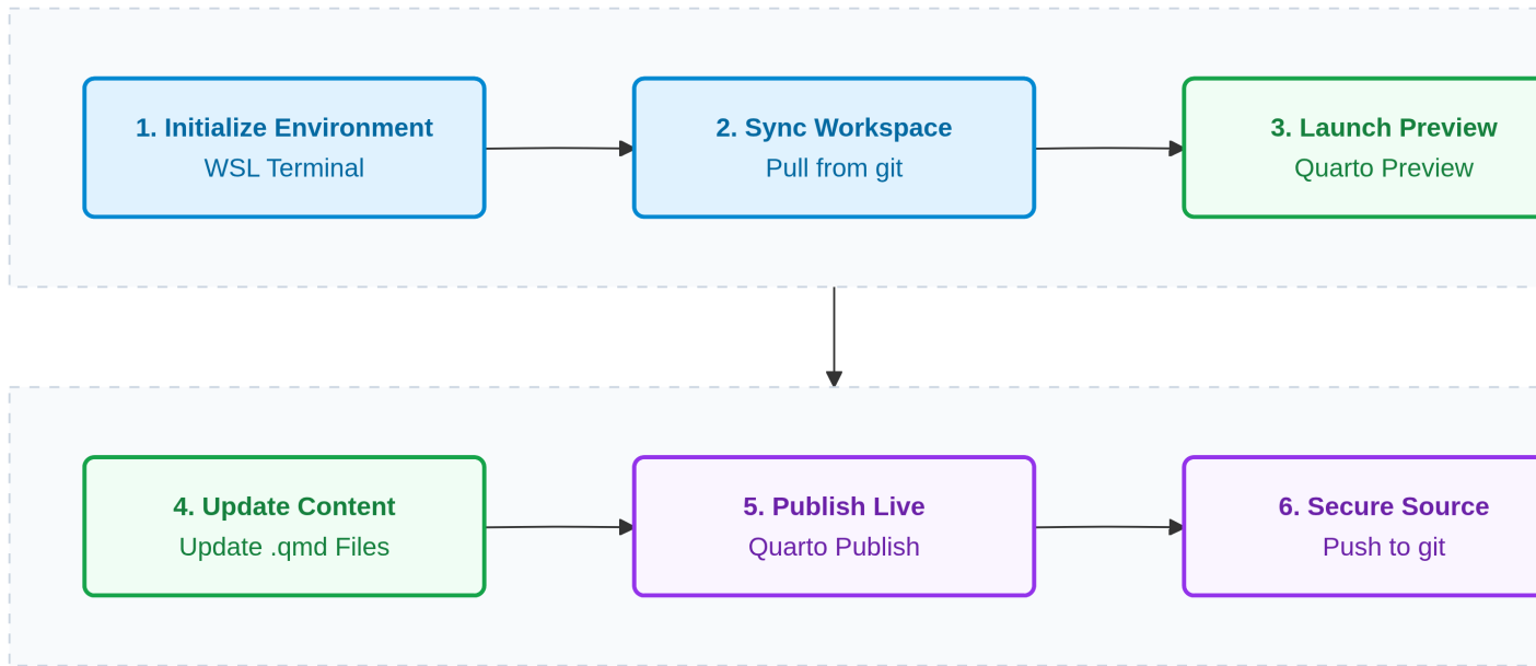
Figure 5.1: Daily Writing and Publishing Workflow
