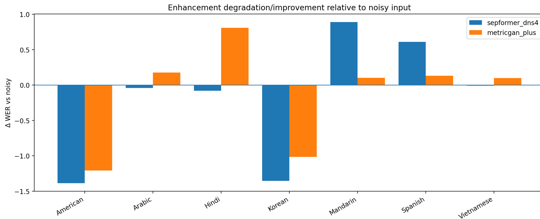
Relative Delta WER vs Noisy
