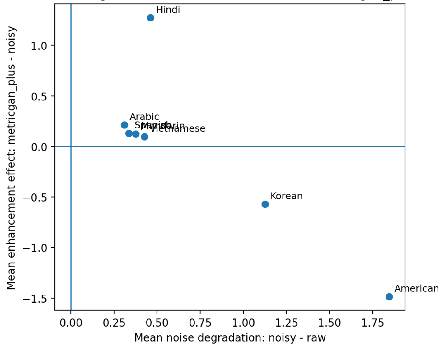
Noise degradation vs enhancement effect: metricgan_plus
