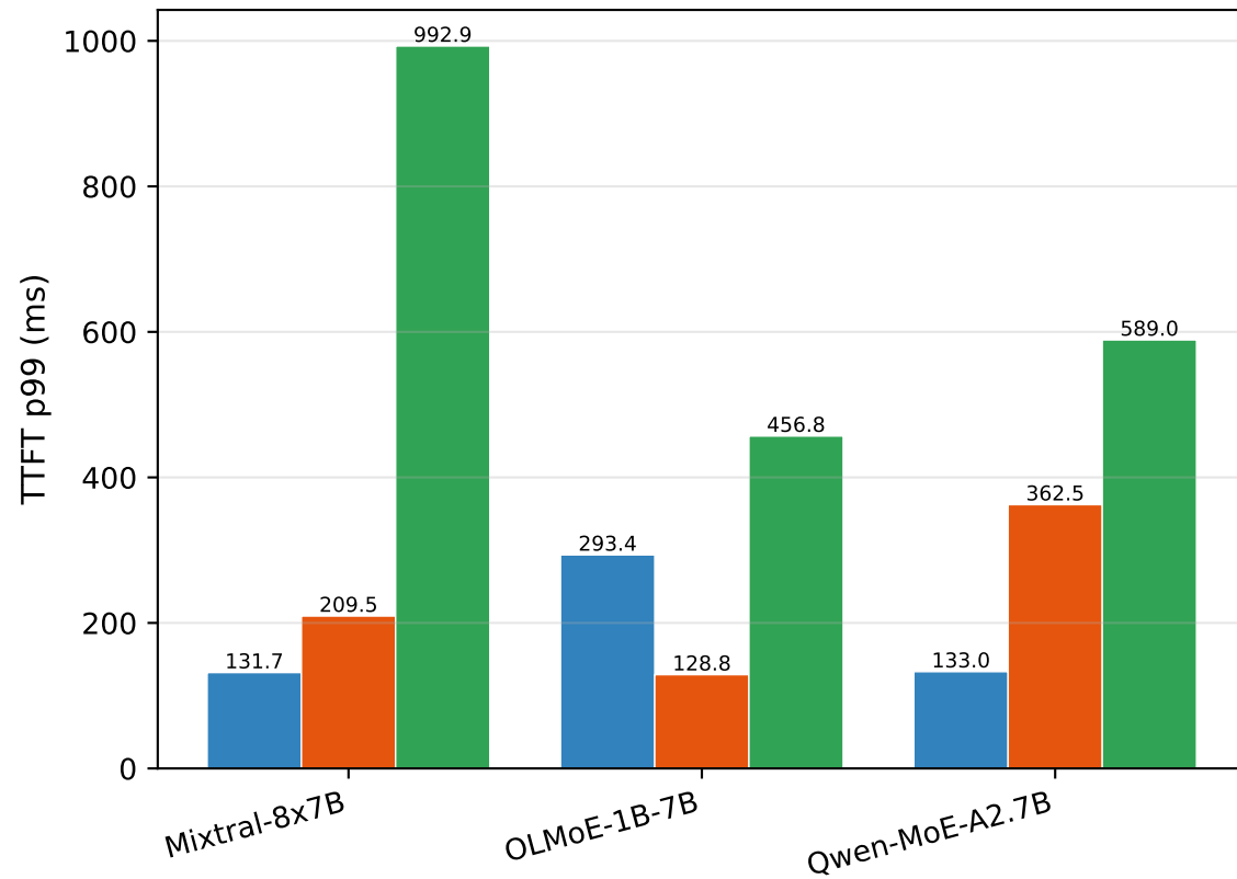
TTFT p99 (tail latency)
