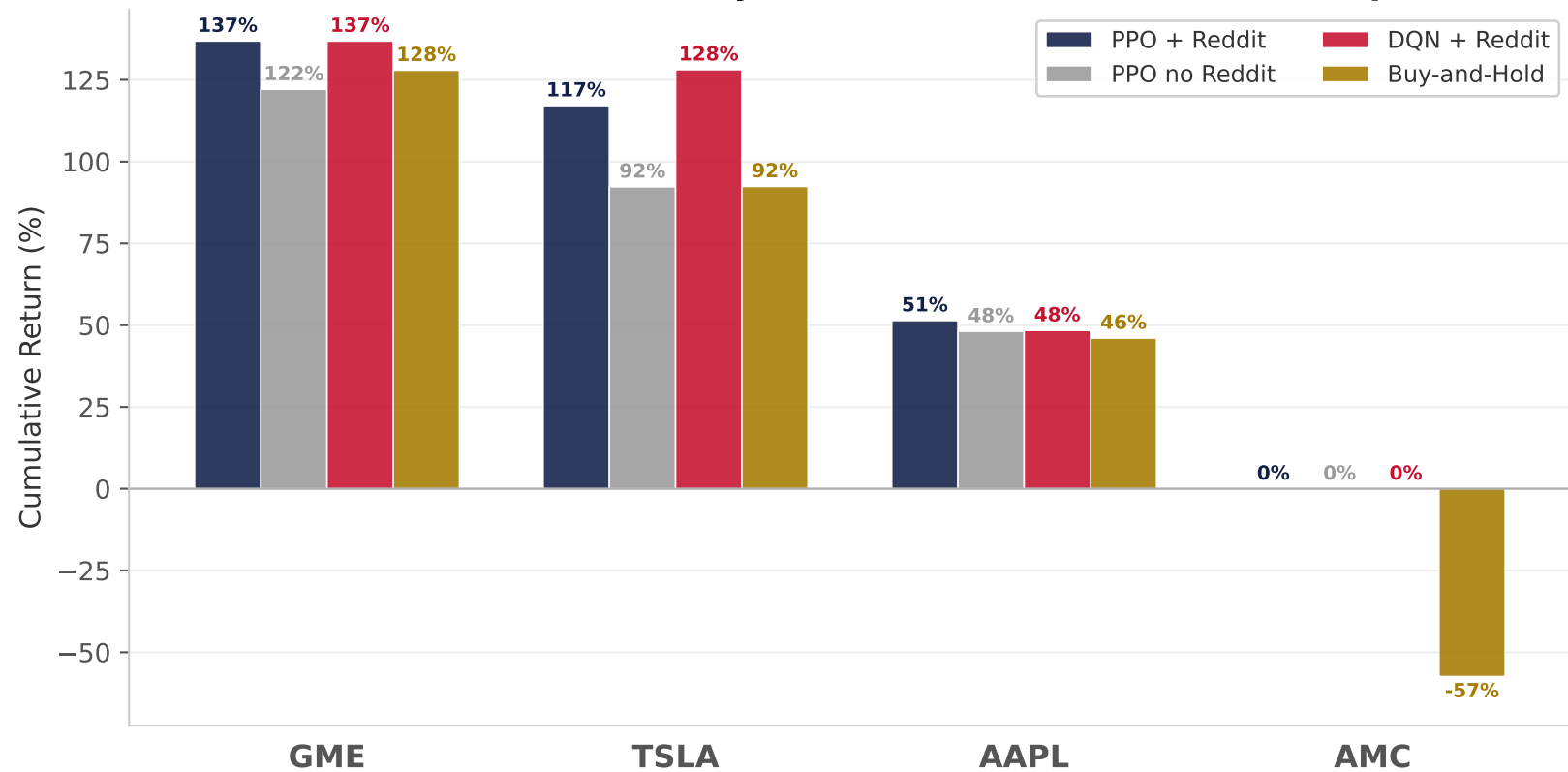
Cumulative Return (%) by Model and Stock — 80/20 Test Split
