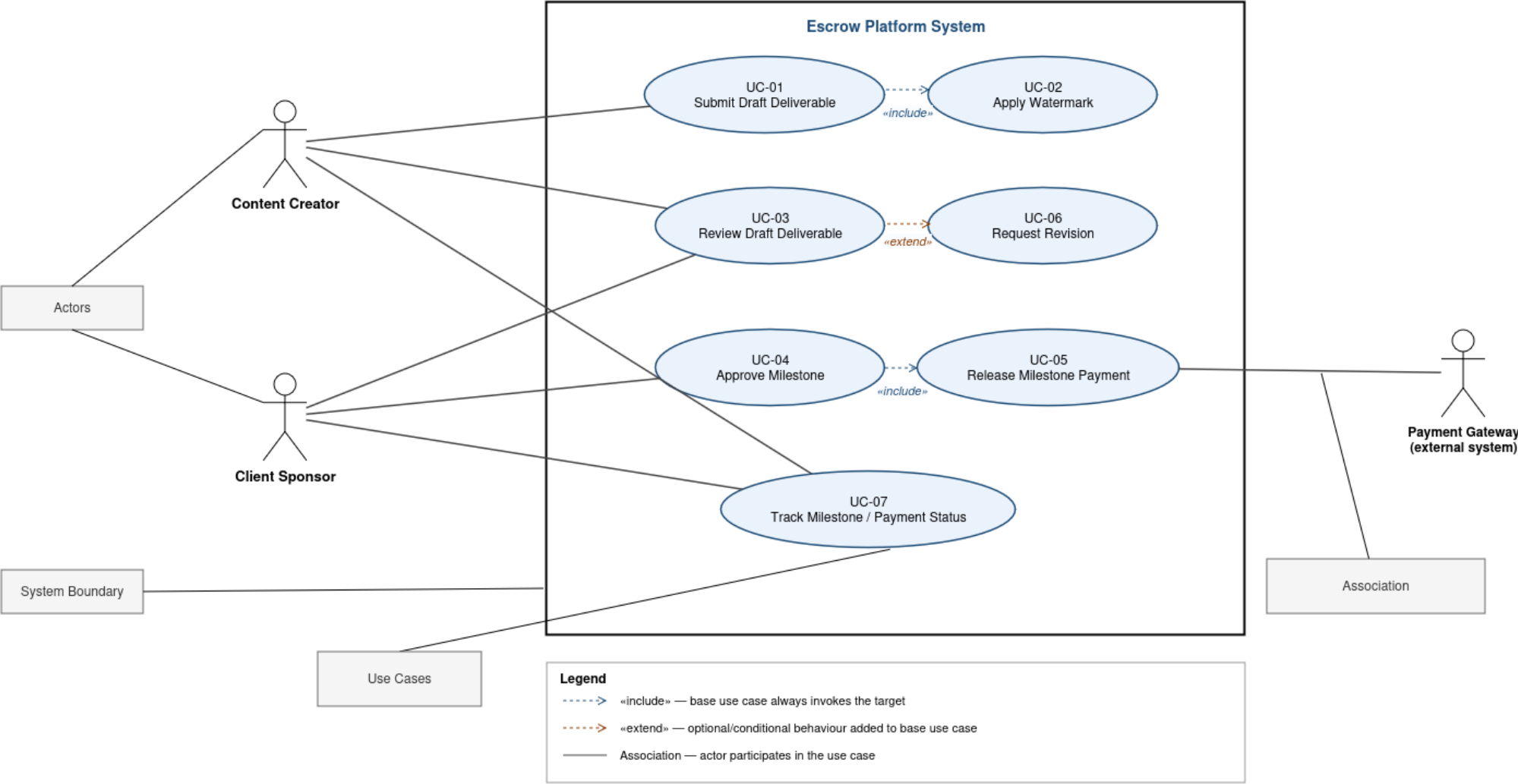
Use-Case Diagram: Freelance Content Creator Escrow Platform
