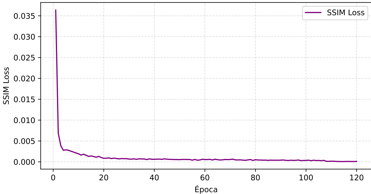
SSIM Loss
