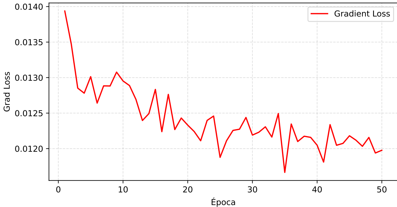
Gradient Loss
