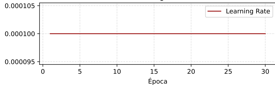
Learning Rate
