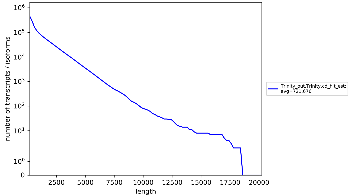
Cumulative transcript / isoform length plot
