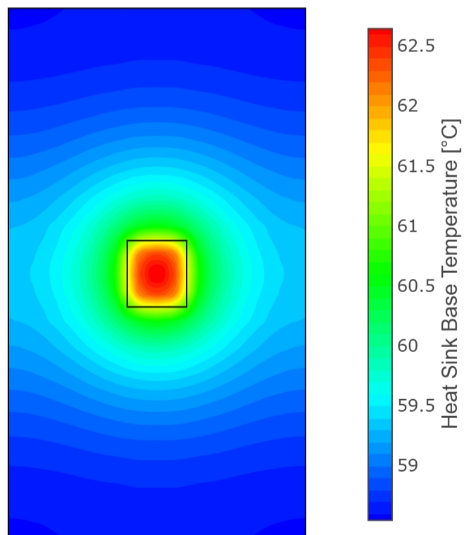
Figure 2. Temperature on the base of the heat sink
