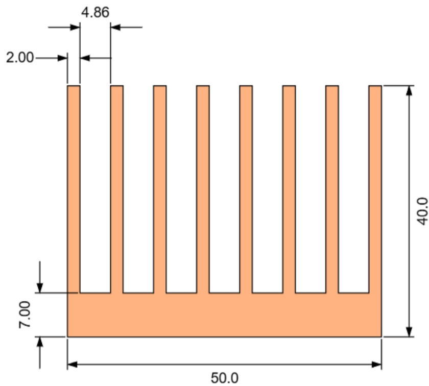
Figure 1. Heat sink dimensions
