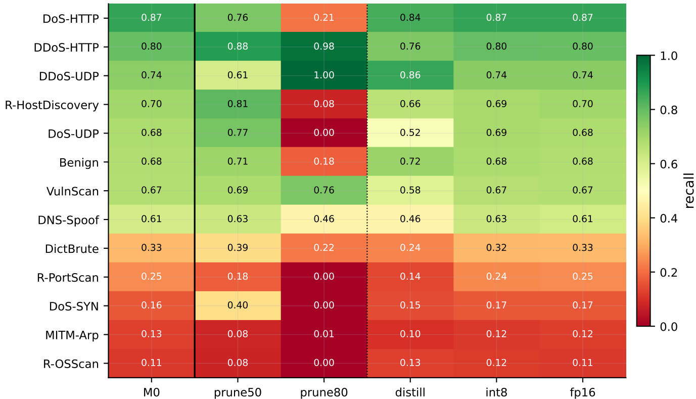
Per-class recall across the compression matrix (CNN, measurable classes)
